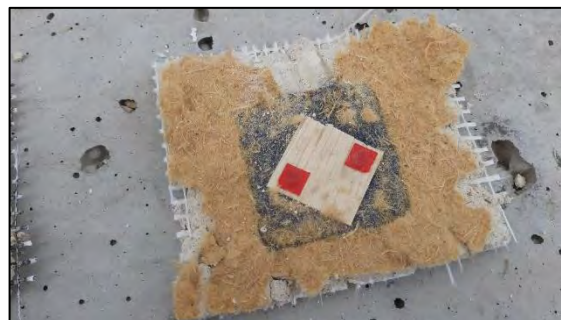
Figure 43: Removed render layer of variant N 2.3 (bright render) with Balsa sensor and wood fibre residues. No fungal mycelium visible.
